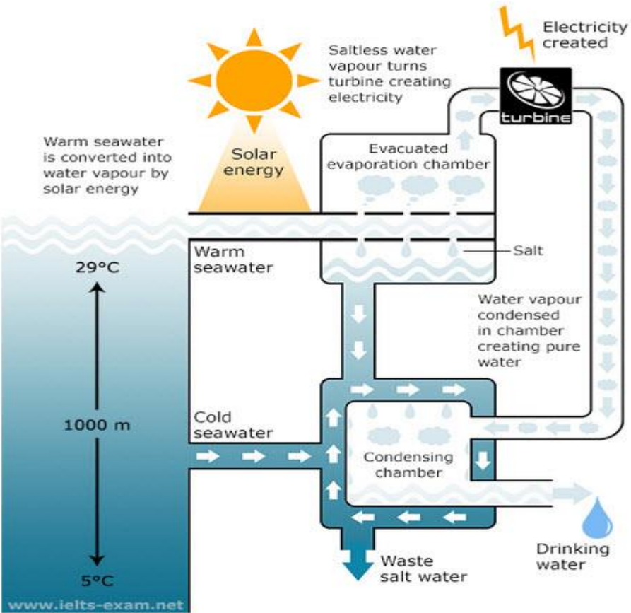
How Ocean Thermal Energy Conversion (OTEC) works
